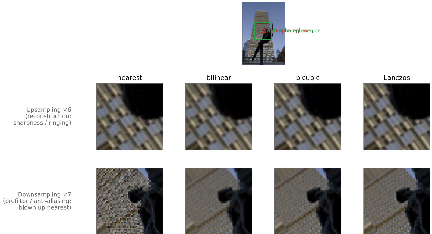
Figure 6.4.16 (reproduced). The kernel ladder on a real photograph, in both regimes, resampled under a 35° rotation (the general case, not a clean axis-aligned zoom). The subject is a near-Nyquist window grid (the Prudential facade) chosen because fine repeating structure is exactly where the kernel choice bites. Top row, upsampling (reconstruction): magnify a small patch and the kernel reconstructs the in-between values: nearest holds each sample as a hard square (blocky), bilinear is smooth but soft, bicubic (Catmull–Rom) restores edge contrast with its negative side-lobes, Lanczos (a windowed sinc) is the sharpest; on smooth natural content bicubic and Lanczos are close, their negative-lobe ringing visible mainly at high-contrast edges. Bottom row, downsampling (prefilter / anti-aliasing): shrink the grid and the kernel must now act as a prefilter (its footprint widened to the new sample spacing). Nearest does not prefilter: it point-samples and the grid aliases into moiré; bilinear, bicubic and Lanczos average over the discarded detail and stay clean. The kernels were implemented explicitly and evaluated in floating point so their true character (including over/undershoot) is preserved, not clamped away.
