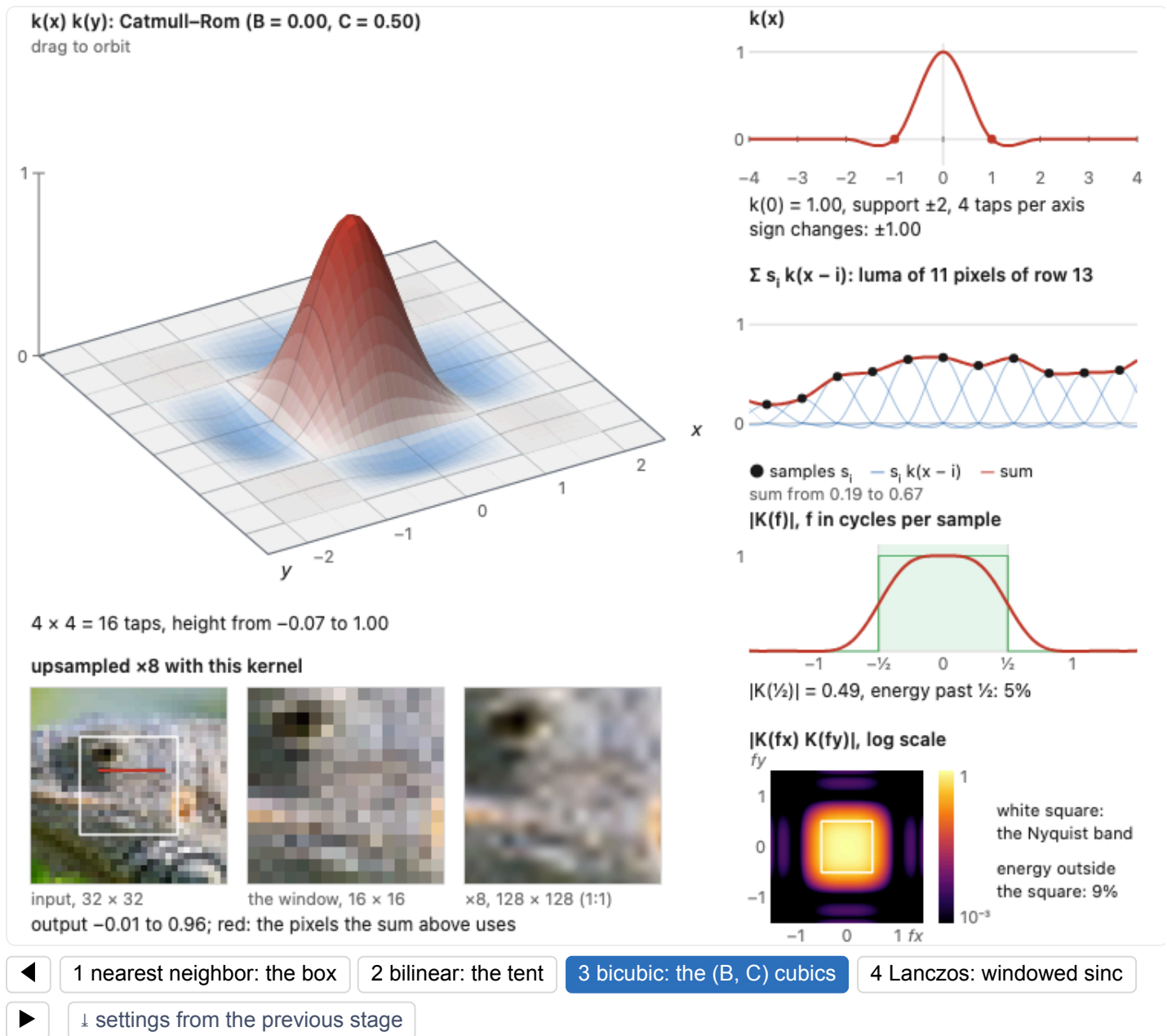
Figure 6.5.7, stage 3 (reproduced). The Mitchell–Netravali cubics k_{BC} in 2-D. The menu sets the named members and the sliders any (B, C) . Below zero the sheet turns blue: Catmull–Rom’s negative lobes are four shallow troughs along the axes, down to -0.07 , and on the diagonals, where both factors are negative, the product is positive again. Catmull–Rom’s reconstruction passes through the samples and overshoots at sharp transitions; the cubic B-spline has no negative lobe, does not overshoot, and misses the samples. The B-spline is the box convolved with itself four times, so its transform is \text{sinc}^4(f) : 0.16 at Nyquist with 0.6% of the energy beyond it, against 0.49 and 4.7% for Catmull–Rom and 0.38 and 3.2% for Mitchell. For every (B, C) the transform is zero at every nonzero integer frequency, because the weights sum to one at every phase.
