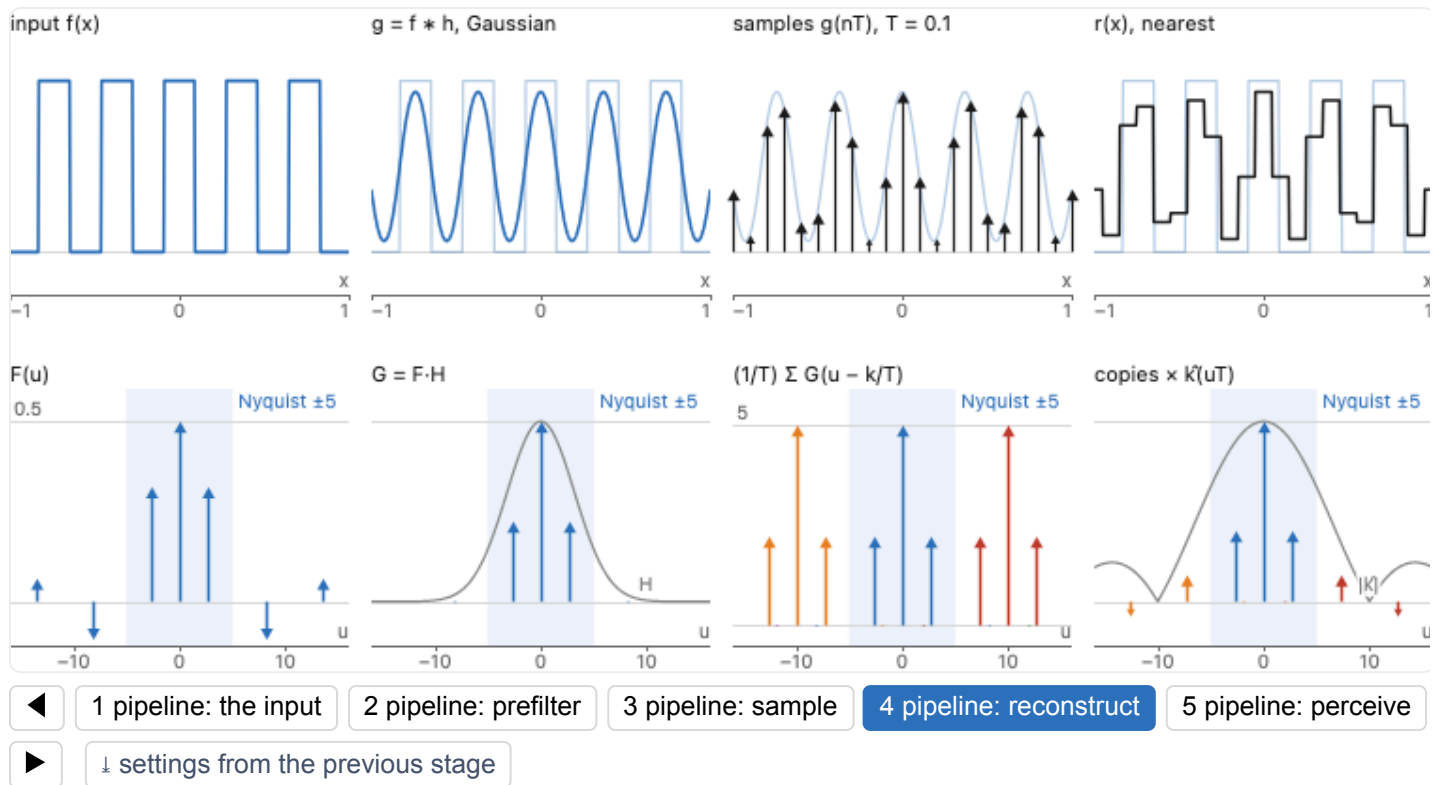
Figure 6.4.9, stage 4 (reproduced). Reconstruction: r(x) = \sum g(nT) k((x - nT)/T) , with the kernel k nearest, linear, cubic (Keys) or a Lanczos-3 windowed sinc, and the input f faint behind. Below, the copies multiplied by the kernel's transform \hat{k}(uT) , its magnitude in gray. The k = 0 copy is the one we want; what survives of the others is imaging, and it is what makes the steps of a nearest reconstruction: at 10 samples per unit the fundamental's first image, at 7.30 cycles per unit, keeps 0.33 of its weight. Linear leaves 0.12 of that image, cubic 0.10 and the windowed sinc 0.004; linear also attenuates the fundamental most (0.76, against 0.87 for nearest, 0.90 for cubic and 0.995 for the windowed sinc).
