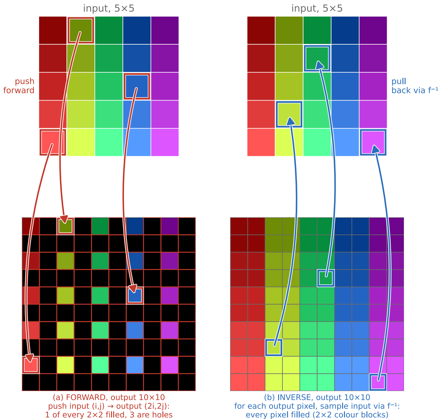
Figure 6.5.2 (reproduced). Forward vs. inverse mapping on a 2× upscale of a small rainbow grid. Left (forward): loop over input pixels and push each to (2i, 2j) ; only one cell of every 2×2 output block gets written, leaving the other three as black gaps (a regular lattice of holes; worse under a rotation, where the holes become tilted slivers). Right (inverse): loop over output pixels and, for each, apply f^{-1} to reach back into the input and sample, so every pixel is filled, no gaps. The arrows trace the two routes for a few pixels: forward arrows start at an input pixel and end where it is written, inverse arrows start at an output pixel and end at the input pixel it reads. The whole chapter loops over the output and reaches back into the input.
