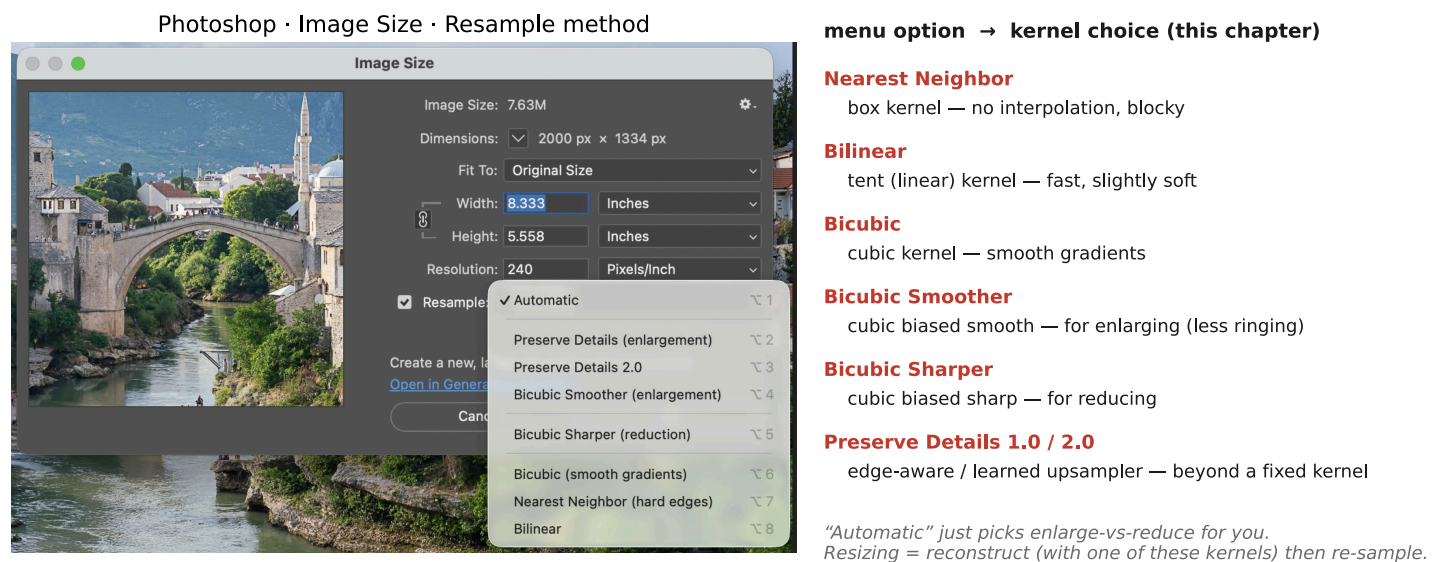
Figure 6.4.14 (reproduced). Adobe Photoshop's Image Size resample-method dropdown (© Adobe Inc., reproduced for educational commentary), with each menu option mapped to its kernel: Nearest Neighbor → box, Bilinear → tent, Bicubic → cubic, Bicubic Smoother → cubic biased smooth (enlarge), Bicubic Sharper → cubic biased sharp (reduce), Preserve Details → an edge-aware / learned upsampler. The shipping product is this chapter's kernel zoo as a menu.
