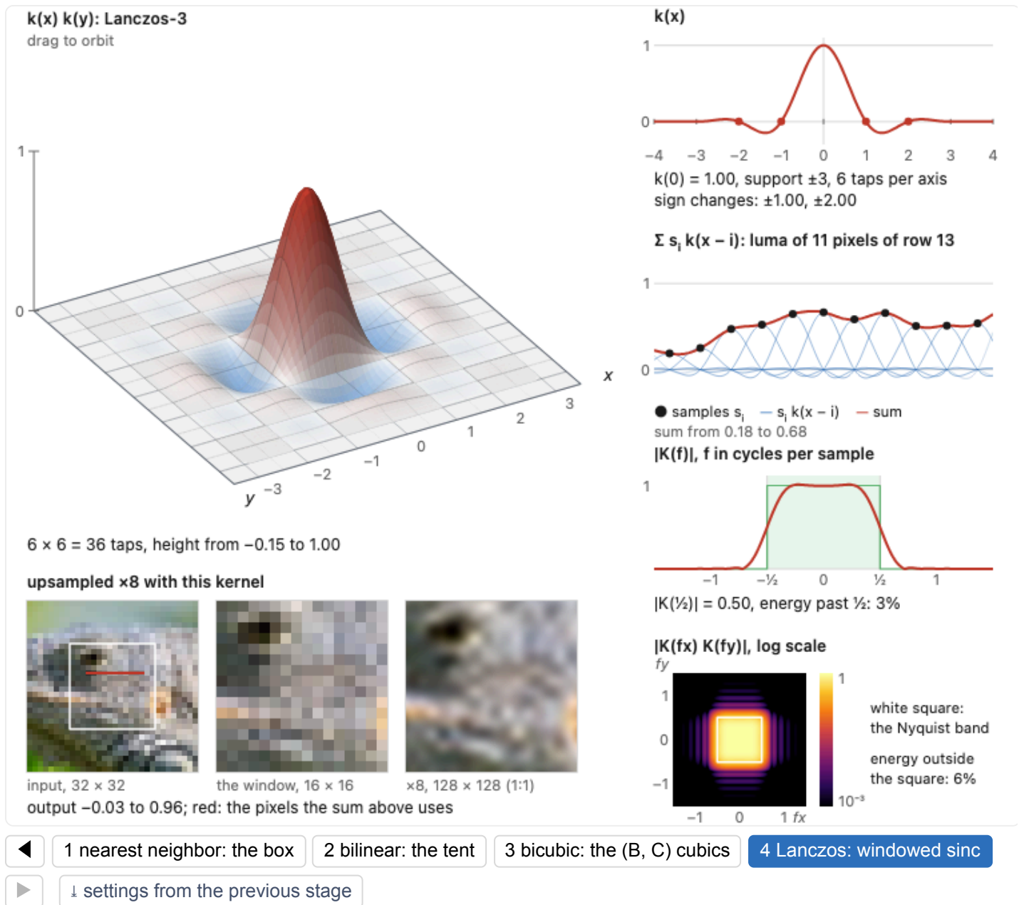
Figure 6.5.7, stage 4 (reproduced). The Lanczos kernel \text{sinc}(x) \text{sinc}(x/a) in 2-D, order a from 2 to 4: 2a taps per axis, 4a^2 in 2-D, and a - 1 sign changes on each side. Its transform is the closest of the four kernels to the ideal: about 0.50 at Nyquist for every order, with 4.6%, 2.9% and 2.1% of the energy beyond Nyquist for a = 2, 3 and 4 (9%, 6% and 4% outside the square in 2-D), and the step from passband to stopband steepens as a grows. The price is the lobes: the 2-D kernel dips to -0.09 , -0.15 and -0.18 , and the reconstruction rings at sharp transitions. The weights are not renormalized here, and Lanczos weights do not sum exactly to one, so a constant row comes back with a ripple of up to 1.9%, 0.6% and 0.2%; practical resamplers renormalize them.
