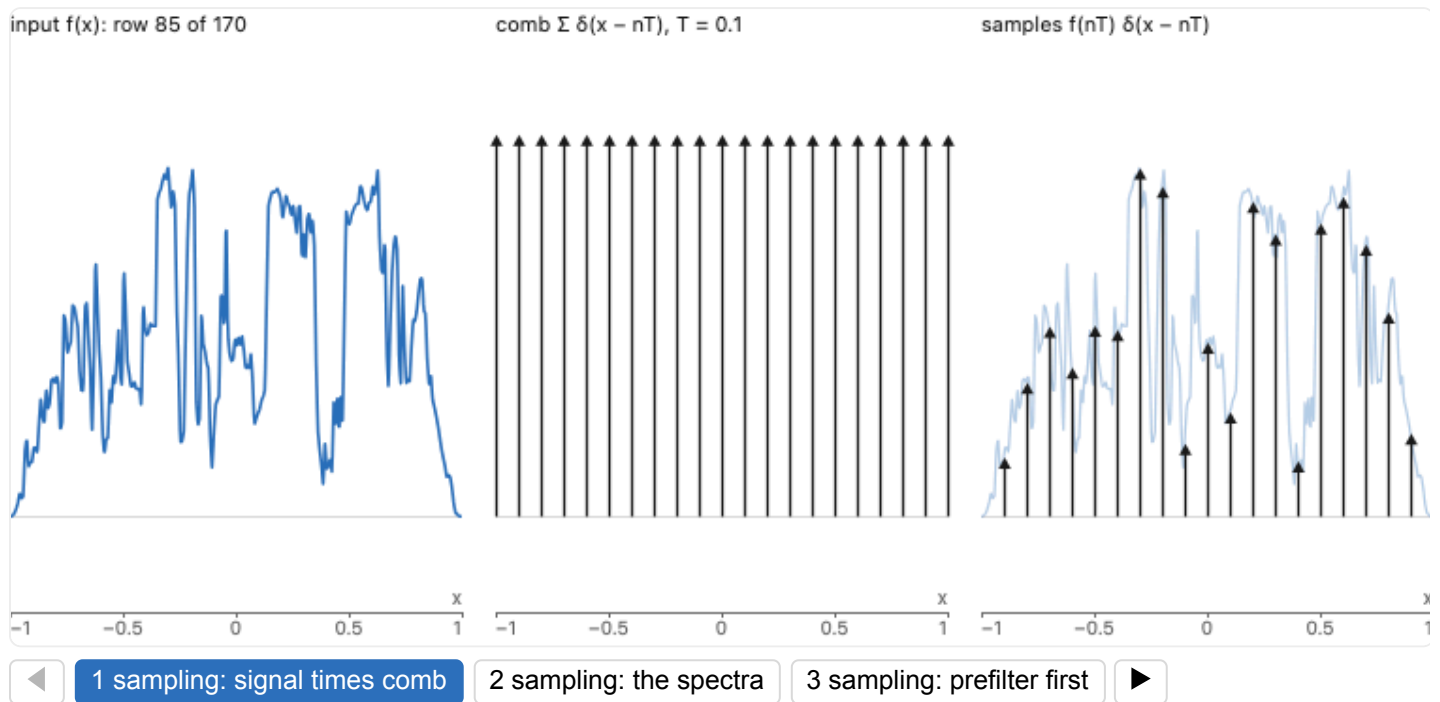
Figure 6.4.4, stage 1 ( reproduced ). Sampling as multiplication by a Dirac comb. Left: the input f(x) , a sine, a box, a sawtooth, a box train, or one row of a photograph (linearly interpolated and tapered at its ends). Middle: the comb \sum \delta(x - nT) , unit Diracs drawn as arrows every T . Right: their product, Diracs of weight f(nT) , with f drawn faintly behind. Change the input, its parameters and the sampling rate 1/T : the arrows on the right are all that remains of f .
