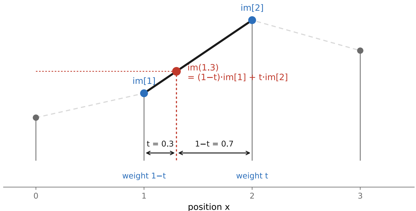
Figure 6.5.3 (reproduced). 1-D linear interpolation. To reconstruct the value at the fractional position 1.3 between samples I[1] and I[2] , blend them in proportion to one minus the distance to each: I[1.3] = 0.7 \cdot I[1] + 0.3 \cdot I[2] . The reconstructed signal is the straight line joining consecutive samples; a neighbor's weight is 1 when you sit on it and falls linearly to 0 a full sample away, the opposite of the raw distance.
