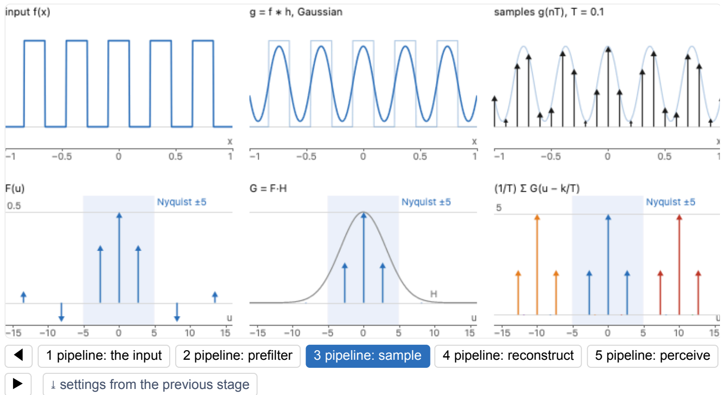
Figure 6.4.9, stage 3 (reproduced). Sampling: Diracs of weight g(nT) , with g faint behind. Below, the samples' spectrum (1/T) \sum G(u - k/T) , one copy of G per multiple of 1/T , each in the color of its tooth in Figure 6.4.4 (blue for k = 0 , red for +1 , orange for -1 , green for +2 , purple for -2 ). Where copies land on the same frequency they add, and an arrow two or more copies share is black. Set the prefilter to none: the box train's third harmonic, at 8.11 cycles per unit, comes back at 1.89 as a red arrow inside the band, and higher harmonics scatter colored arrows across it. That is aliasing.
