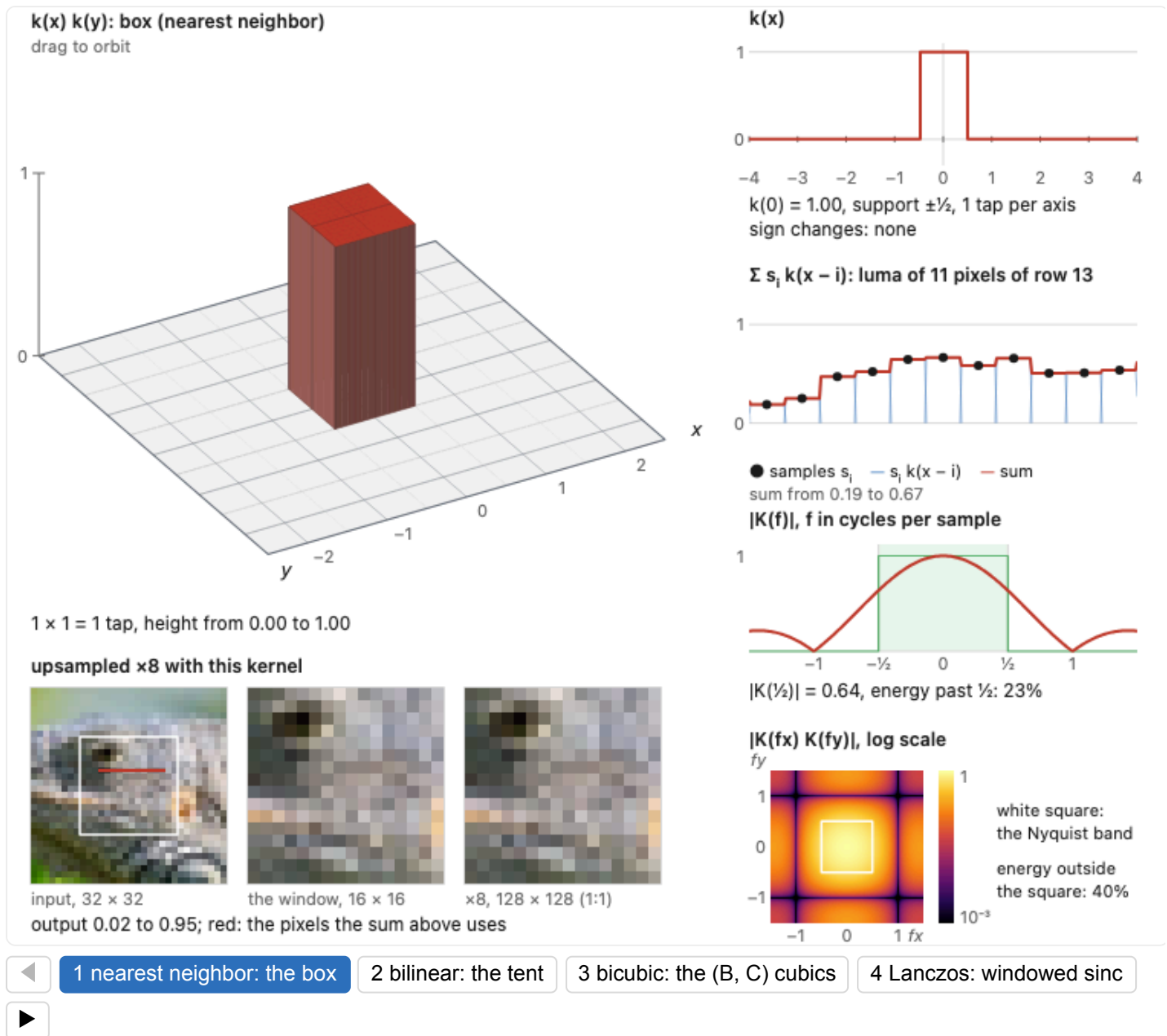
Figure 6.5.7, stage 1 (reproduced). The box kernel of nearest neighbor, k(x) = 1 for |x| < \frac{1}{2} , as the separable 2-D kernel k(x) k(y) : a column one sample wide and of height 1 over the grid of sample positions. Drag the height field to turn it. On the right, top to bottom: the profile k(x) , with a dot wherever the kernel changes sign; eleven pixels of one row of the input (their luma, marked red on the input below) reconstructed as a sum of copies of the kernel, each centered on a sample and scaled by its value (blue); the magnitude of the Fourier transform along f_y = 0 against the ideal reconstruction filter (green), which passes every frequency up to Nyquist, half a cycle per sample, and none beyond; and the 2-D magnitude |K(f_x) K(f_y)| on a log scale, with the Nyquist square outlined. Bottom left, the input, a 16 × 16 window of it, and that window upsampled ×8 with the same kernel, shown at 1:1. The menu picks the input, the same six as Figure 6.5.1 , the iguana first. The box's transform is \text{sinc}(f) : already down to 0.64 at Nyquist, it leaves 23% of its energy beyond Nyquist in 1-D and 40% outside the square in 2-D, the aliasing that shows as blocks.
