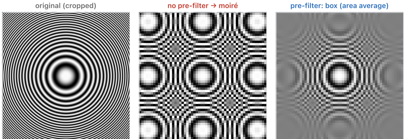
Downsampling \times 4 : pre-filtering reduces aliasing; residual moiré and ringing depend on the filter. The panels use the same crop, fixed to the widest filter support.
