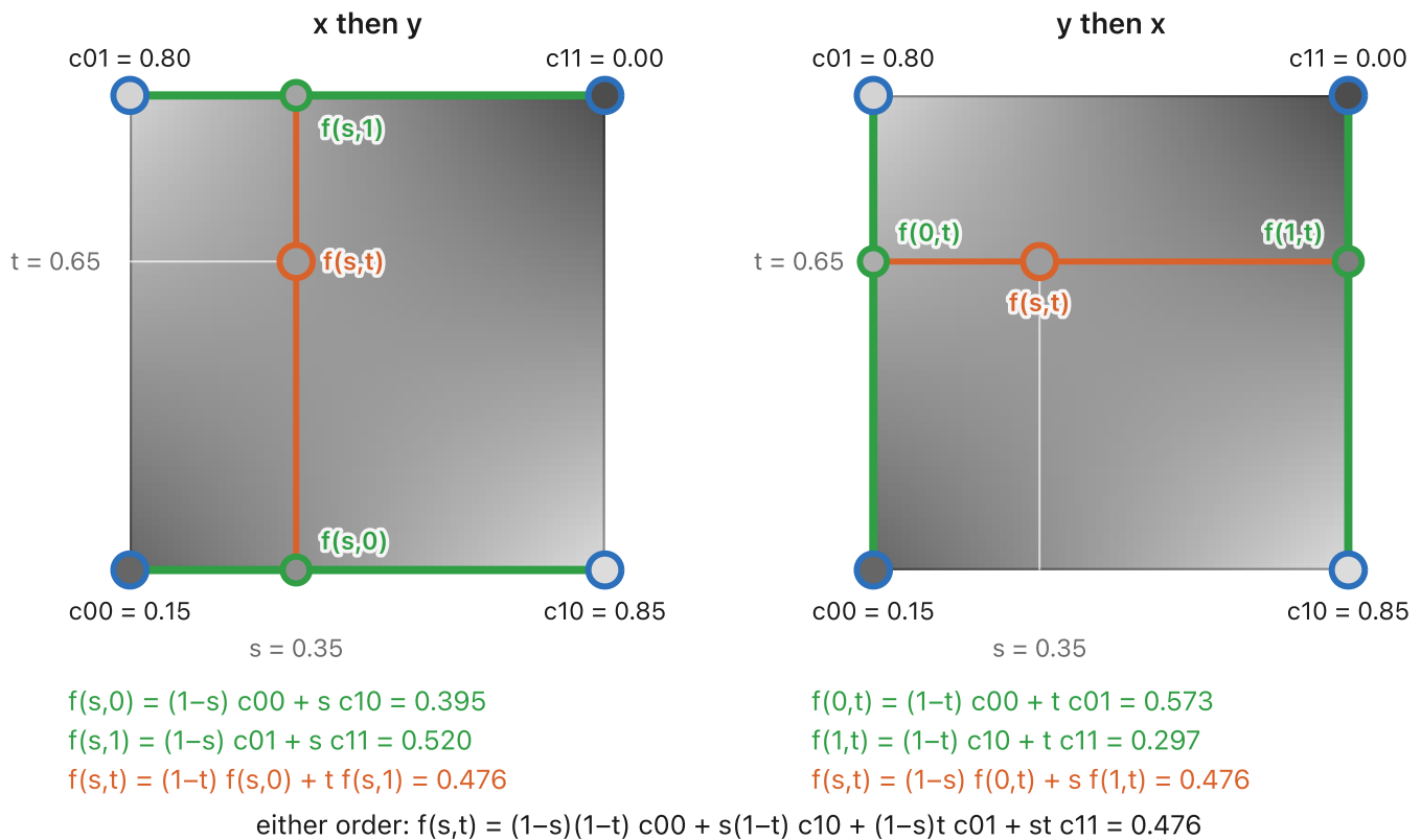
Figure 6.5.4 (reproduced). Bilinear interpolation as two 1-D passes, in both orders (interactive). The query (s, t) falls inside the unit square spanned by its four nearest input pixels, c_{00} to c_{11} ; each square is shaded with the interpolated values. On the left we interpolate along x first, on the bottom and top edges (green), f(s, 0) = (1 - s) c_{00} + s c_{10} and f(s, 1) = (1 - s) c_{01} + s c_{11} , then along y between those two (orange). On the right we interpolate along y first, on the left and right edges, f(0, t) and f(1, t) , then along x . The intermediate values differ, the result does not: both orders expand to (1 - s)(1 - t) c_{00} + s(1 - t) c_{10} + (1 - s)t c_{01} + st c_{11} , four weights that are products of the x - and y -blend factors, linear in each axis, hence bilinear. Drag the query point in either square, or set the corner values; the defaults are those of the height field that follows.
