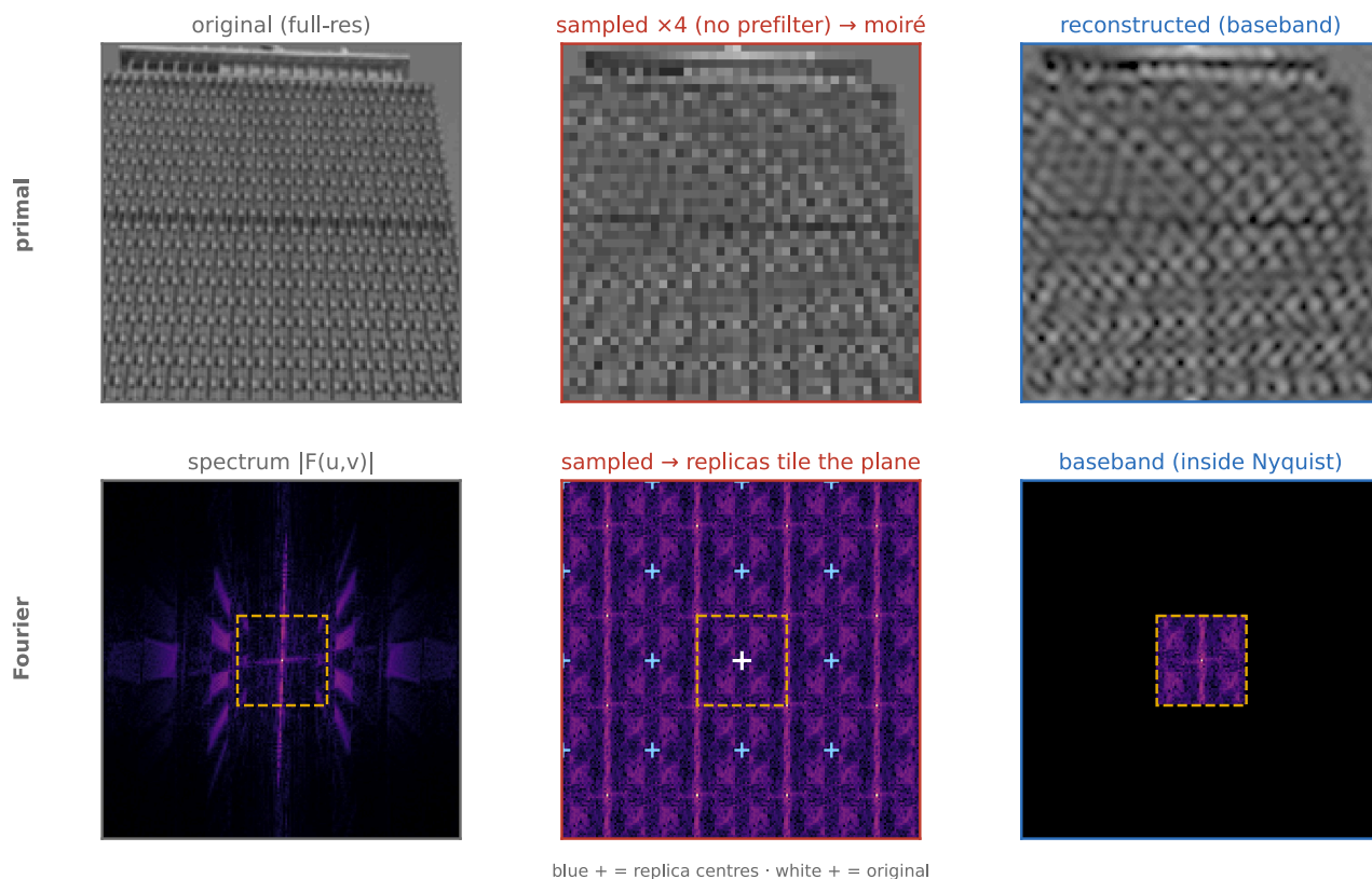
Figure 6.4.3 (reproduced). Aliasing is directional in 2-D. A regular 2-D pattern (a near-periodic grid and a slanted edge), point-sampled on a coarse grid without a prefilter, aliases in ways 1-D cannot: the grid's high spatial frequency folds to a low frequency of a different orientation, so the moiré bands run in a direction unrelated to the windows that caused them, while the slanted edge breaks into the canonical stair-step / "jaggies." A 2-D frequency carries a direction as well as a rate, and aliasing folds both, which is why 2-D moiré appears in unexpected directions. The cure is the same as in 1-D: prefilter (area-average) before sampling.
