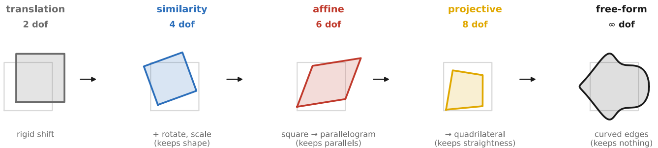
Figure 11.1.3 (reproduced). The degrees-of-freedom ladder. A unit square under, left to right, translation (2) → similarity (4) → affine (6) → projective (8) → free-form (∞). Each rung adds freedom and breaks a preserved property: similarity keeps shape, affine keeps parallelism (square → parallelogram), projective keeps only straightness (square → quadrilateral, parallels converging), and free-form keeps nothing globally.
