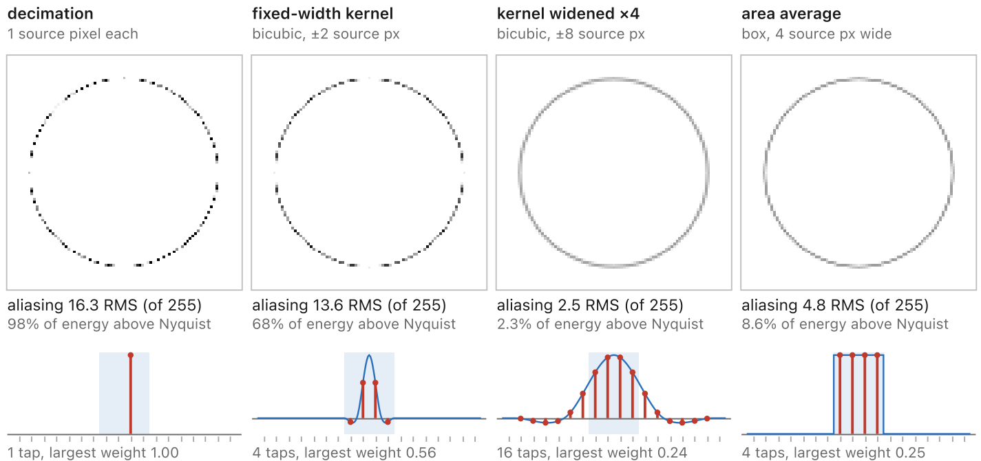
Figure 6.5.12 (reproduced). Four downsamplers on one input, side by side, each with the kernel it applies drawn under it in source pixels: the dots are the weights one output pixel takes from the source pixels (the ticks), and the shaded band is that output pixel's footprint, s source pixels wide. Decimation reads one source pixel. A fixed-width kernel, bilinear or bicubic at the source's own scale, reads two to four pixels near the middle of the footprint and ignores the rest, the default of several of the libraries Parmar et al. compare on a thin circle. The kernel widened by the factor covers the footprint, and so does the area average. On the thin circle the first two break the line into scattered dots; on the zone plate they bring back rings that are not in the source. The readout under each result measures its aliasing: the part of the source above the output's Nyquist frequency (what an ideal low-pass in the DCT basis removes) is passed through the same downsampler, and whatever comes out is content the output cannot hold. It is given as an RMS in 8-bit code values and as a share of that part's energy. At 1/4 on the circle with bicubic, decimation keeps 98% of it, the fixed kernel 68%, the area average 8.6% and the widened kernel 2.3%. At odd whole factors the fixed tent lands on a single source pixel and becomes decimation; at other factors its taps shift from one output pixel to the next. The readout measures aliasing, not blur: the widened tent scores lowest and is also the softest. The arithmetic is on sRGB code values, as the libraries do, and each result is enlarged by a whole number with nearest neighbor. Peacock photograph by Bernard Spragg (CCO).
