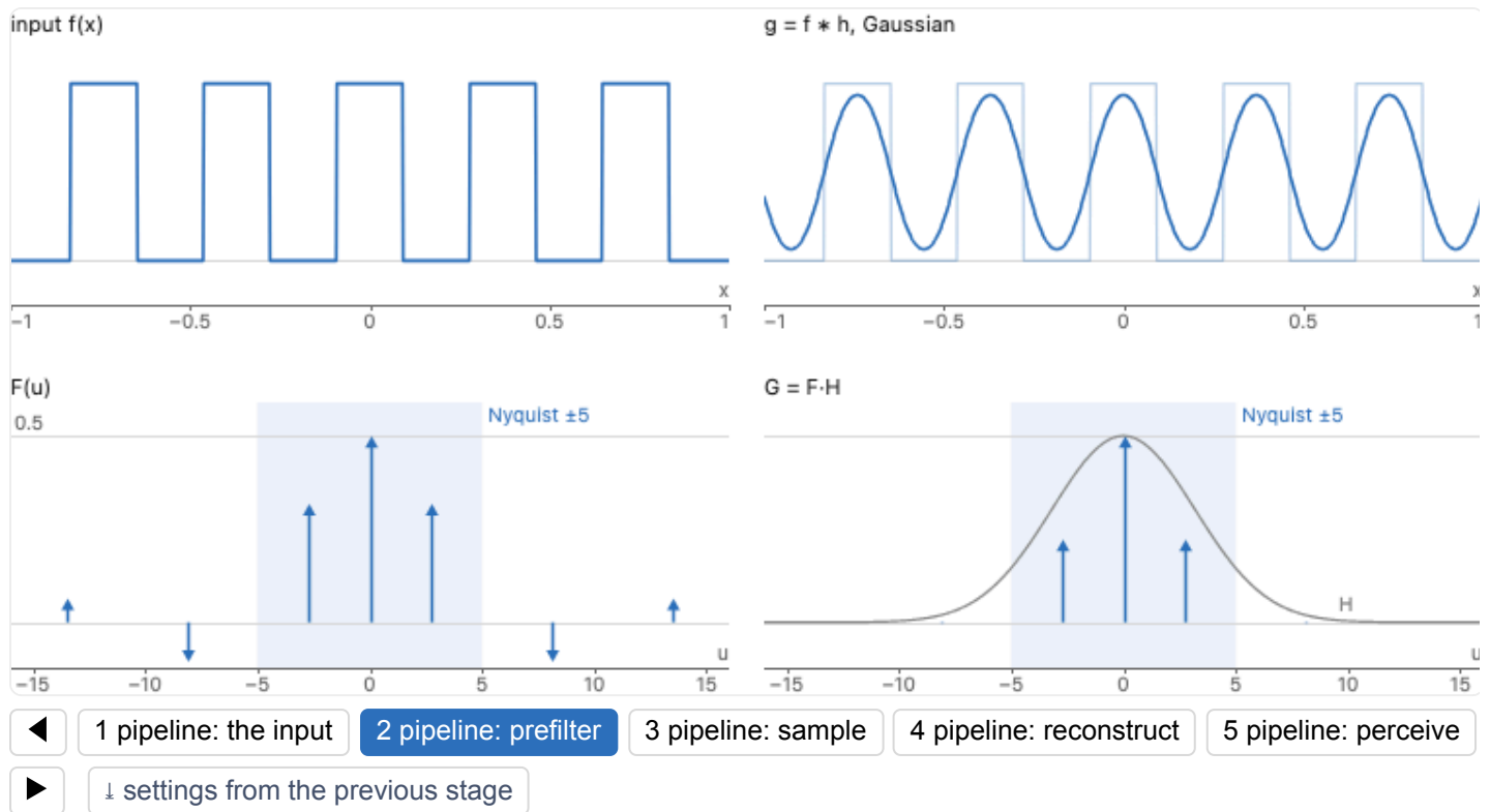
Figure 6.4.9, stage 2 (reproduced). The prefilter, g = f * h , with h tied to the sample spacing T : a box of width T , a Gaussian of standard deviation T/2 , or a Lanczos-3 windowed sinc scaled by T . Below, G = F \cdot H , with H in gray on a scale where the top rule is 1, and the Nyquist band \pm 1/(2T) shaded. The stage opens on the Gaussian, which at 10 samples per unit keeps 0.70 of the box train's fundamental (2.70 cycles per unit) and 0.04 of its third harmonic (8.11). Switch the filter and move the rate to see what each keeps inside the band and lets through beyond it.
