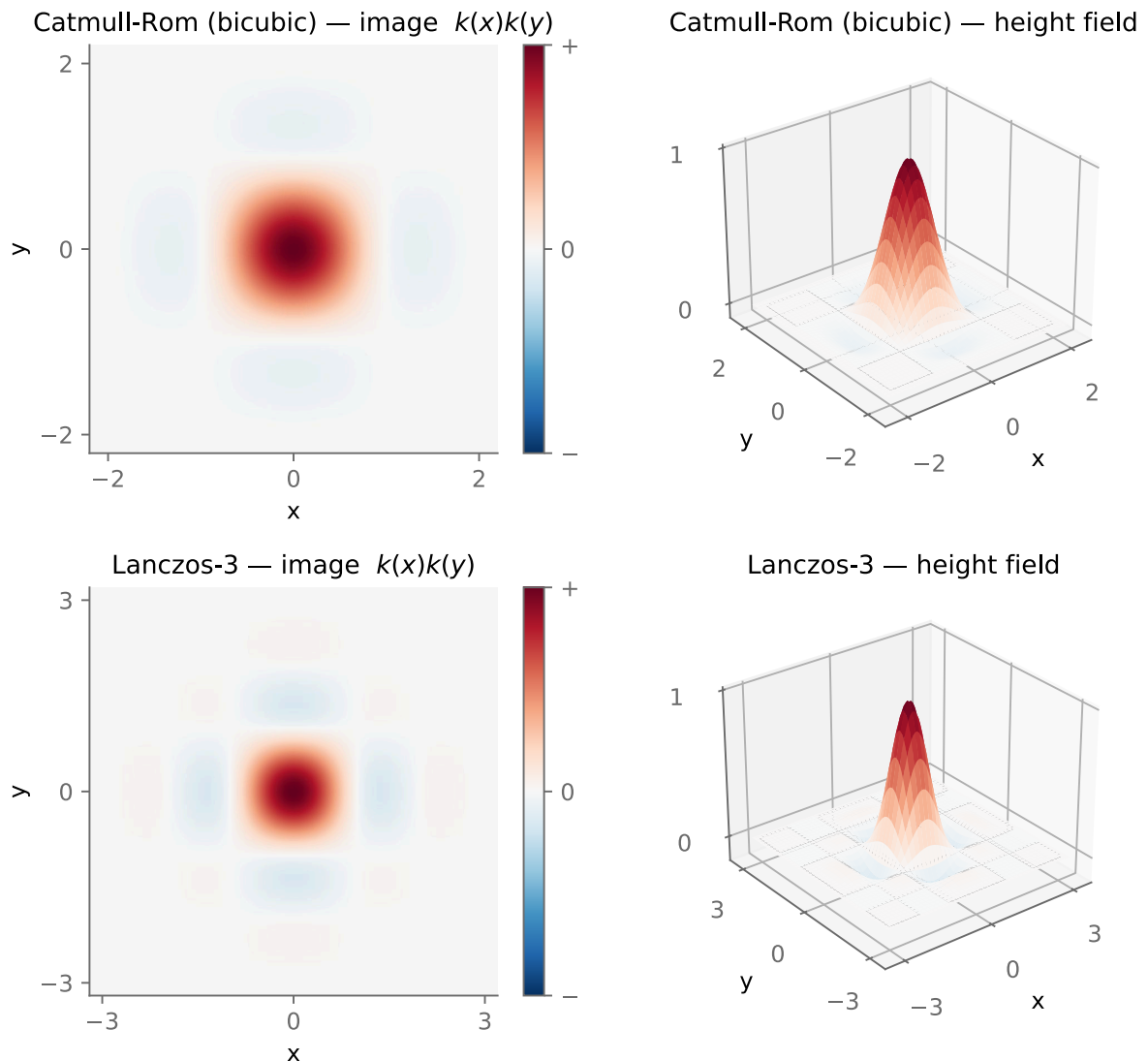
Figure 6.4.13 (reproduced). The kernels in 2-D, formed as the separable outer product k(x) k(y) for Catmull–Rom and Lanczos-3, each shown as a diverging-color image and as a height field. The smooth central mound is ringed by a shallow negative moat, the sharpening side-lobes seen from above.
