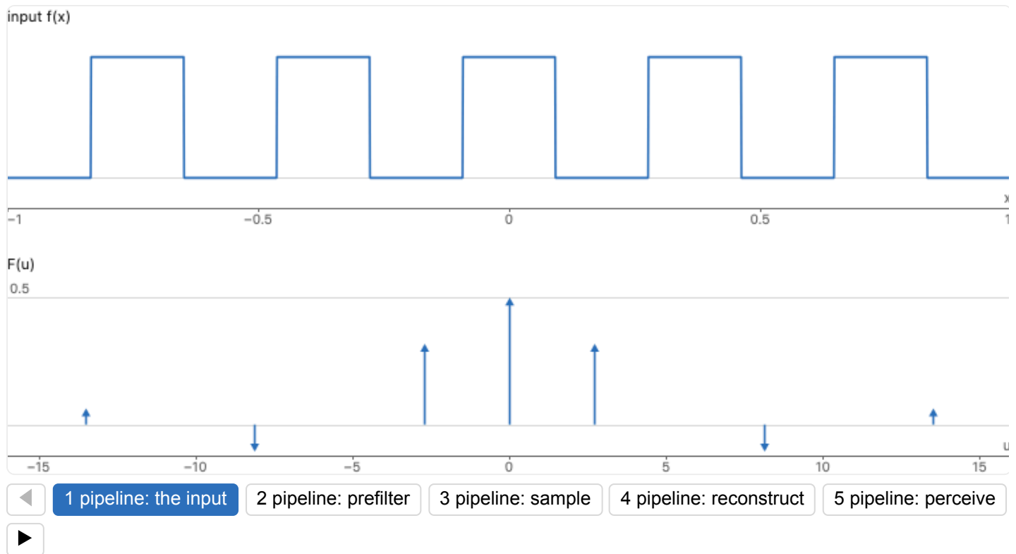
Figure 6.4.9, stage 1 ( reproduced ). The sampling pipeline in one dimension, one column per step, each signal above and its Fourier transform below ( u in cycles per unit length). The first column is the input: a box train (period 0.37, half on, the default), a sine, a box, a sawtooth, or one row of a photograph. Periodic inputs have Diracs for spectra, drawn as arrows; real spectra are drawn signed, the others as magnitudes.
