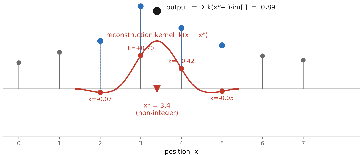
Figure 6.5.6 (reproduced). Why the kernel must be a continuous function. A row of discrete input samples sits on the integer grid; a smooth kernel k(x) is centered at a non-integer query location x^* between two of them, and the output is the sum of each sample times the kernel's height at that sample's offset. Because the center is fractional, those offsets are fractional too, so the kernel has to be a closed-form curve readable at any real argument, not a fixed stencil of integer taps.
