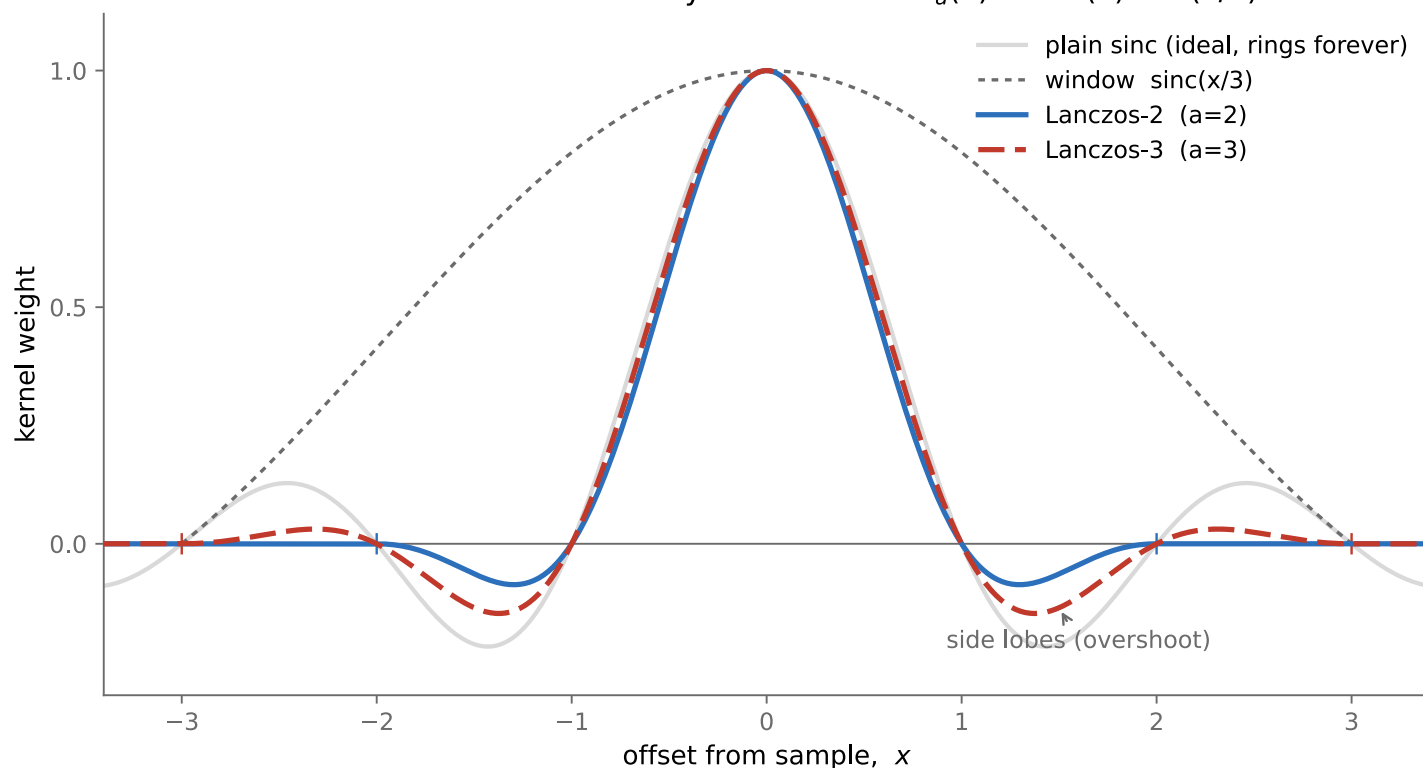
Figure 6.4.11 ( reproduced ). The Lanczos kernel \text{sinc}(\pi x) \text{sinc}(\pi x/a) over its a -sample support (Lanczos-2 and Lanczos-3) against the plain infinite sinc: a tall central lobe flanked by alternating side-lobes, truncated at \pm a , closest to the ideal box spectrum, but the surviving side-lobes are what produce edge ringing.
