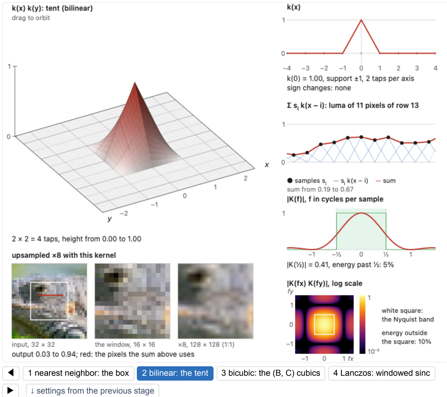
Figure 6.5.7, stage 2 (reproduced). The tent, k(x) = 1 - |x| for |x| < 1 , in 2-D. The product k(x) k(y) is not a pyramid: along a diagonal it falls as (1 - t)^2 , and its four taps are the four bilinear weights. The reconstruction of the row is the polyline through the samples. Its transform is \text{sinc}^2(f) , 0.41 at Nyquist, so the passband droops more than the box's, while only 5% of the energy lies beyond Nyquist in 1-D and 10% outside the square in 2-D.
