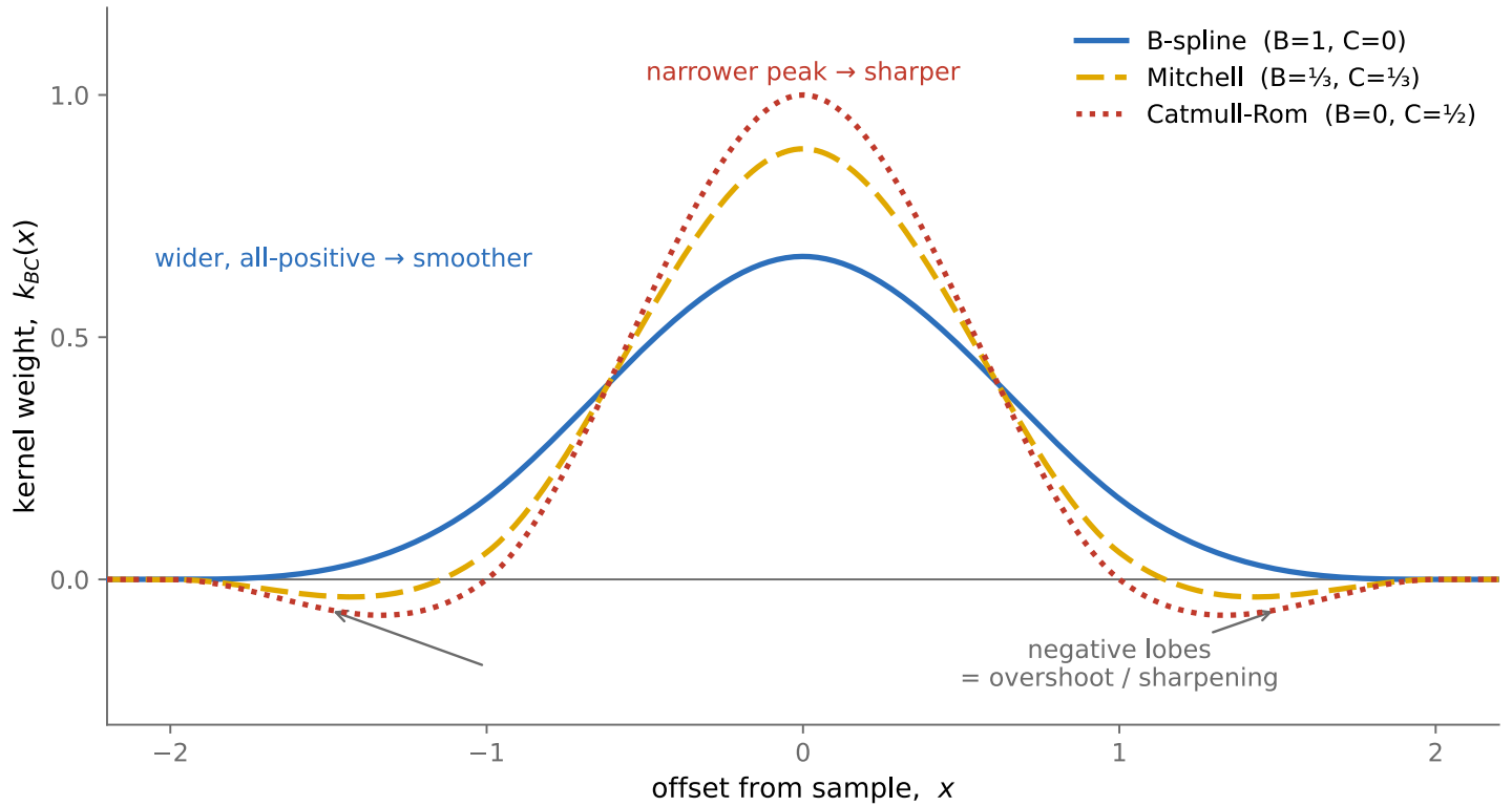
Figure 6.4.12 (reproduced). The cubic kernel k_{BC}(x) as a one-parameter-pair family, plotted for the three standard members: cubic B-spline (B, C) = (1, 0) , all-positive and smooth; Catmull–Rom (0, \frac{1}{2}) , interpolating with strong negative side-lobes; and Mitchell–Netravali (\frac{1}{3}, \frac{1}{3}) , the balanced default between them. The deeper the negative lobes, the sharper (and ringier) the reconstruction.
