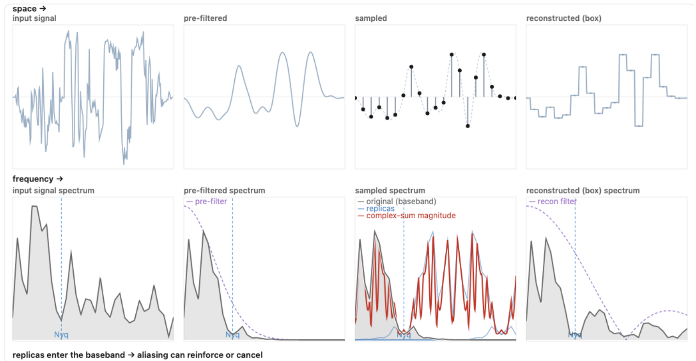
Figure 6.4.5 (reproduced). Interactive (1-D): sampling, aliasing, and the pre-filter. An input, by default the same image scanline as Figure 6.4.4 (the middle row of the old-town rooftops), or a periodic signal (a sine, square or sawtooth at a frequency you choose), is shown with its samples; drag the sampling rate and watch the reconstructed signal alias to a lower frequency the moment you drop below Nyquist (two samples per cycle), with both the signal and its spectrum (the replicated spectral copies) drawn side by side. Where replicas overlap, the spectrum shows the magnitude of their complex sum, which includes reinforcement and cancellation; the magnitudes of overlapping copies do not simply add. Toggle the anti-aliasing pre-filter (a low-pass blur applied before sampling) and watch the offending high frequencies attenuated before they can fold: the alias fades, at the cost of a little blur. A Gaussian or other finite filter attenuates rather than strictly band-limits, so some alias can remain. Tick marks mark the sample locations.
