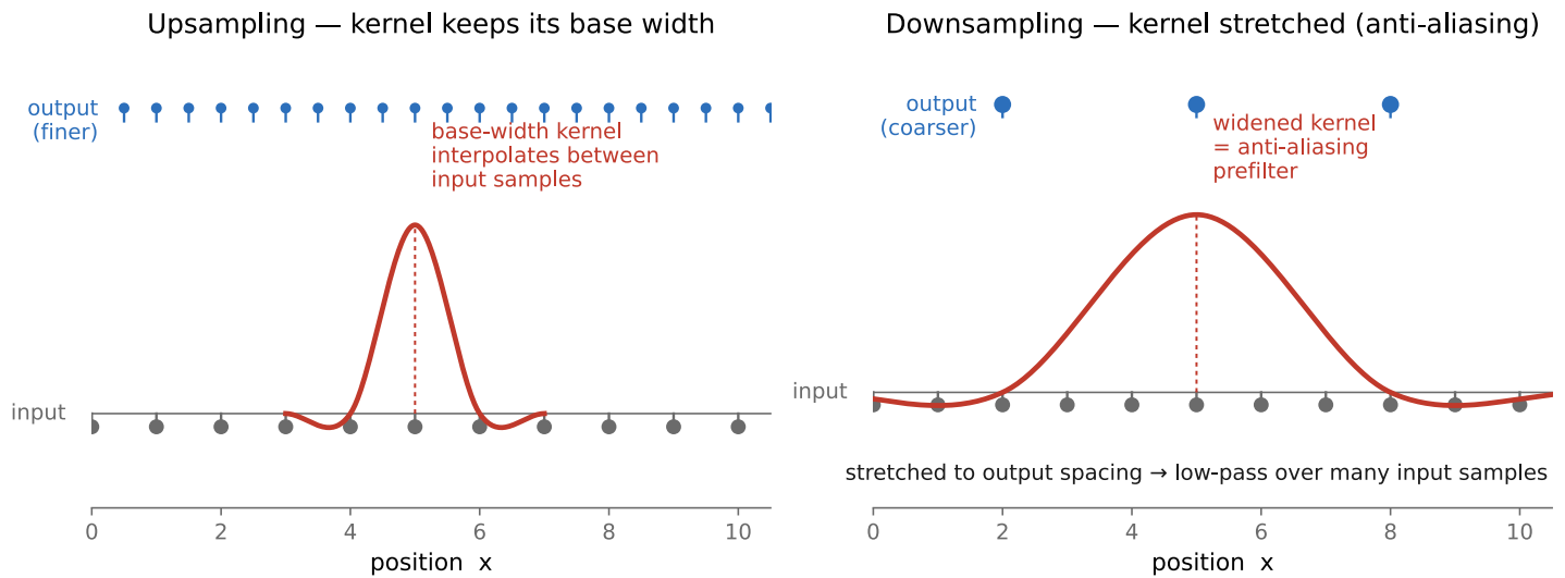
Figure 6.5.11 (reproduced). The one knob that distinguishes up- from downsampling. Upsampling: the kernel keeps its native width in input space (about four pixels for bicubic), reaching across the same handful of dense input samples no matter how much you enlarge. Downsampling: the kernel is stretched to span the output-pixel spacing, by s\times for an s\times reduction, so it averages over all the input detail crammed into each new pixel, doubling as the anti-aliasing prefilter. Same kernel shape, scaled differently.
