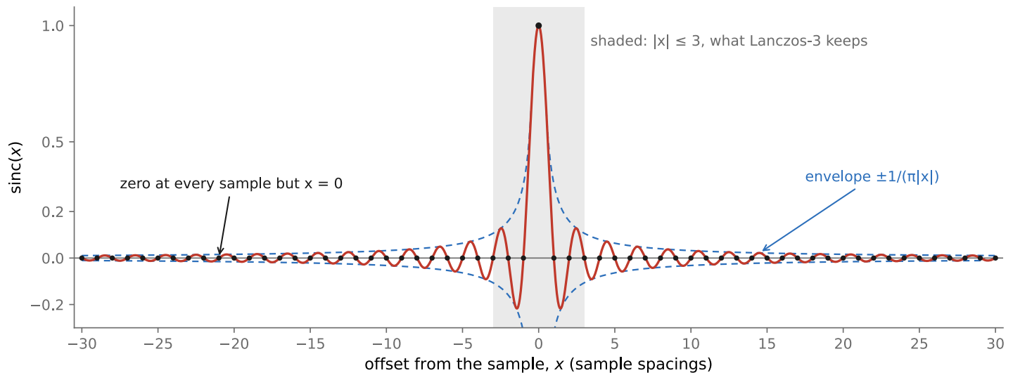
Figure 6.4.10 (reproduced). The sinc, \text{sinc}(x) = \sin(\pi x)/(\pi x) , over 30 sample spacings on each side. It is 1 at its own sample and 0 at every other one (dots), and between them it oscillates with alternating sign, the lobes shrinking only as 1/(\pi|x|) (dashed envelope): the lobe near x = 30 is still about 1% of the peak. The shaded band, |x| \leq 3 , is the part of it that Lanczos-3 keeps.
