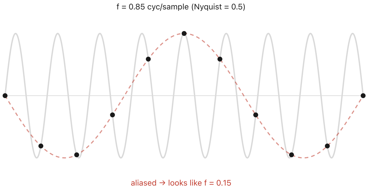
Figure 6.4.1 ( reproduced ). Sampling a sine too coarsely \rightarrow aliasing. A high-frequency sinusoid (light) is sampled at too few points per cycle; the samples (dots) are consistent with a completely different, lower-frequency sinusoid (dark), its alias. Below twice the signal's frequency (the Nyquist rate) the two are indistinguishable from the samples alone: the high frequency "folds" down and masquerades as a low one. This is the moiré / wagon-wheel effect.
