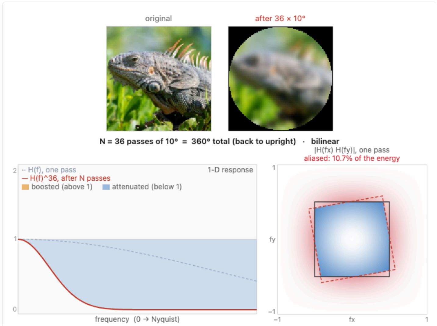
Figure 6.5.16 (reproduced). The rotation challenge, interactive. Rotate one image to a chosen total angle in equal steps, each step re-sampling the previous result with the selected filter (nearest · box · bilinear · Lanczos · bicubic). The rotation runs on sRGB code values, and "box" here has two-pixel support, unlike nearest-neighbor. The orientation depends only on the total; the damage depends on the number of passes N and on the filter: drop the step size to compound more passes, switch filters to watch nearest jitter, box and bilinear blur to mush, and Lanczos or a well-tuned bicubic hold the detail. For bicubic, drag the (B, C) point to choose the cubic. Set the total to 360^\circ to land back at the original orientation and read off pure resampling loss. A bottom panel plots the kernel's 1-D frequency response H(f) and, as an approximation of the N stacked passes, H(f)^N : the curve collapsing toward DC is why detail vanishes: each pass multiplies the spectrum by H , so after N passes the surviving spectrum is roughly H^N . The plot keeps one scale, 0 to 2, and shades orange where the passes boost a frequency (the sharpening that rings) and blue where they attenuate it. The square panel is the 2-D spectrum of the separable kernel, |H(f_x)H(f_y)| , out to one cycle per sample, with the source grid's Nyquist square in black and the turned grid's dashed. Only frequencies inside both pass as themselves; what the kernel lets through elsewhere, shown red, comes from the spectrum's copies or from corners the turned grid cannot hold, and folds back as aliasing. The readout gives its share of the kernel's energy: about 29% for nearest and 8% for Lanczos at a 10^\circ step. Switched to N passes, the panel multiplies the kernel turned by every step, and only what fits inside every grid along the way passes as itself, outlined dashed: the square rounds into a near disc of radius one half, and the readout gives both the share left outside after all the passes and the share a single pass aliases.
