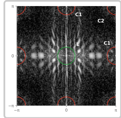
log spectrum of the mosaic: luma at the centre (green), C1 on the axes and C2 in the corners (red), each ringed at its carrier
