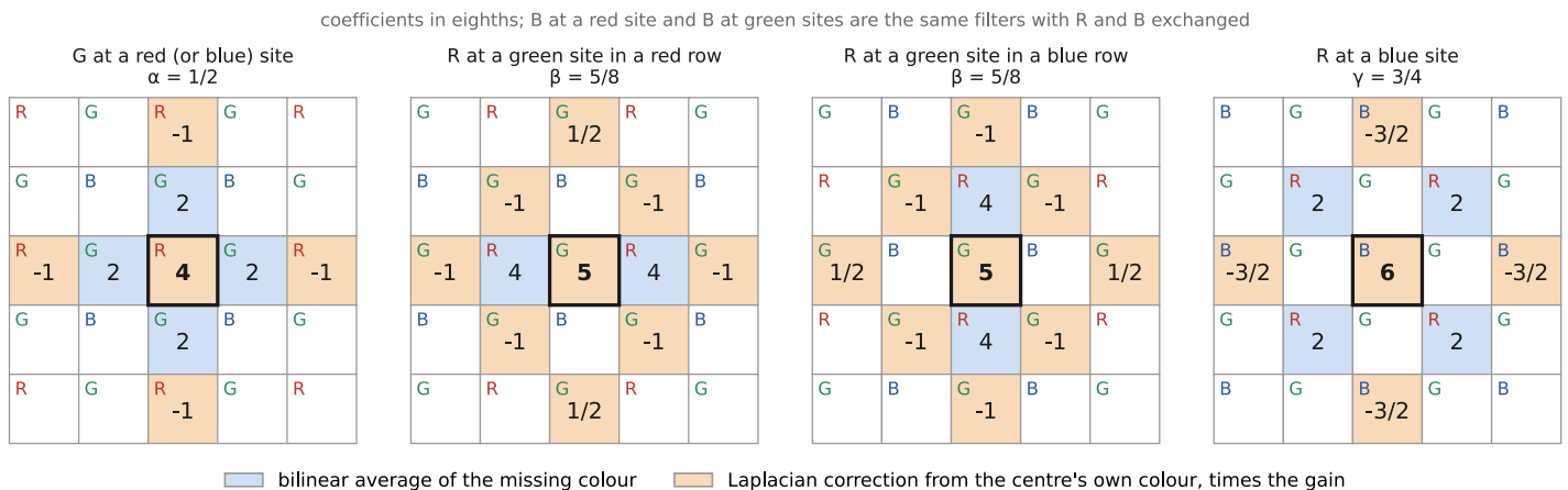
Figure 15.2.3 (reproduced). The four Malvar–He–Cutler filters, in eighths: green at a red or blue site, red at a green site in a red row and in a blue row, and red at a blue site (blue at a red site is the same by symmetry). Each cell shows its weight and the mosaic color it applies to. The bilinear part is shaded blue and the Laplacian correction from the center channel orange, with the published gains \alpha = 1/2 , \beta = 5/8 and \gamma = 3/4 .
