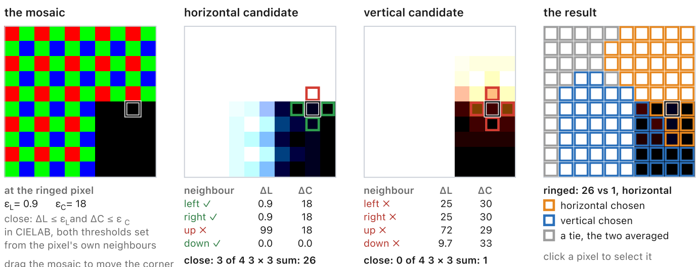
Figure 15.2.5 (reproduced). AHD's homogeneity criterion at one pixel. Left, the mosaic. Then the horizontal and the vertical candidate, the ringed pixel's four neighbors outlined green when they are within both thresholds, \epsilon_L in lightness and \epsilon_C in color (CIELAB), and red when they are not; beneath each, the differences, the count and its sum over 3 \times 3 . The thresholds are the same for both candidates, set from the pixel's own neighbors along each candidate's direction. Right, the result: each pixel framed orange where the horizontal candidate won, blue where the vertical one did, gray on a tie. Next to an edge, the candidate that interpolated across it has made colors that neither side has, and its neighbors stop matching. The inputs are the corner, a sine grating, a Siemens star and a zone plate (both band-limited), the maze's colored stripes, and crops of four photographs, on a grid of 10 \times 10 or 16 \times 16 . Interactive: choose the input and the grid, set the pattern's angle, period, spokes or frequency, drag on the mosaic to move the pattern or pan the photograph, and click a pixel to test it.
