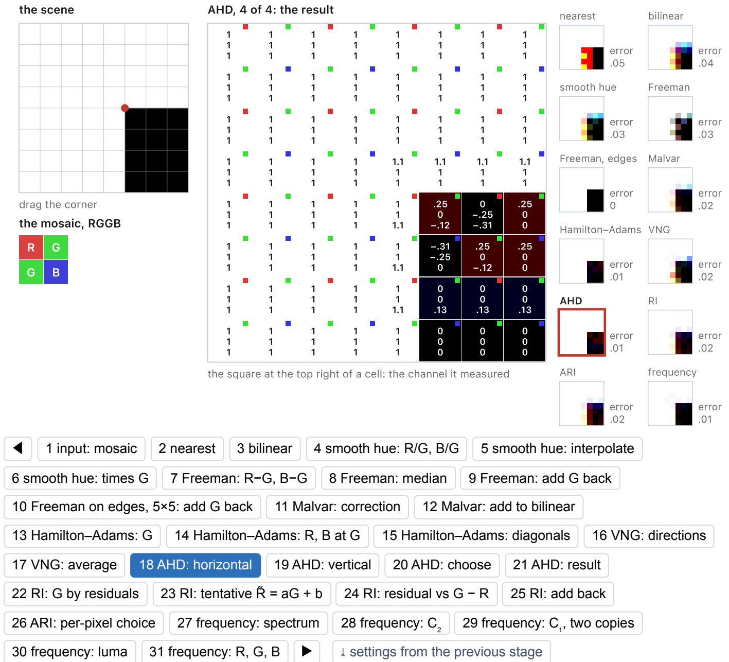
Figure 15.2.2, stage 18 (reproduced). AHD: the horizontal candidate, the vertical candidate, the choice at each pixel from their homogeneity counts summed over 3 \times 3 , and the result. The published method finishes with a median of the color differences; the checkbox adds one, Freeman's 5 \times 5 . Interactive: the same controls, and a checkbox that follows the result with Freeman's 5 \times 5 median; the stages step through the four steps.
