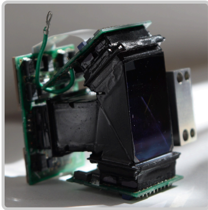
the real 3-CCD prism block
