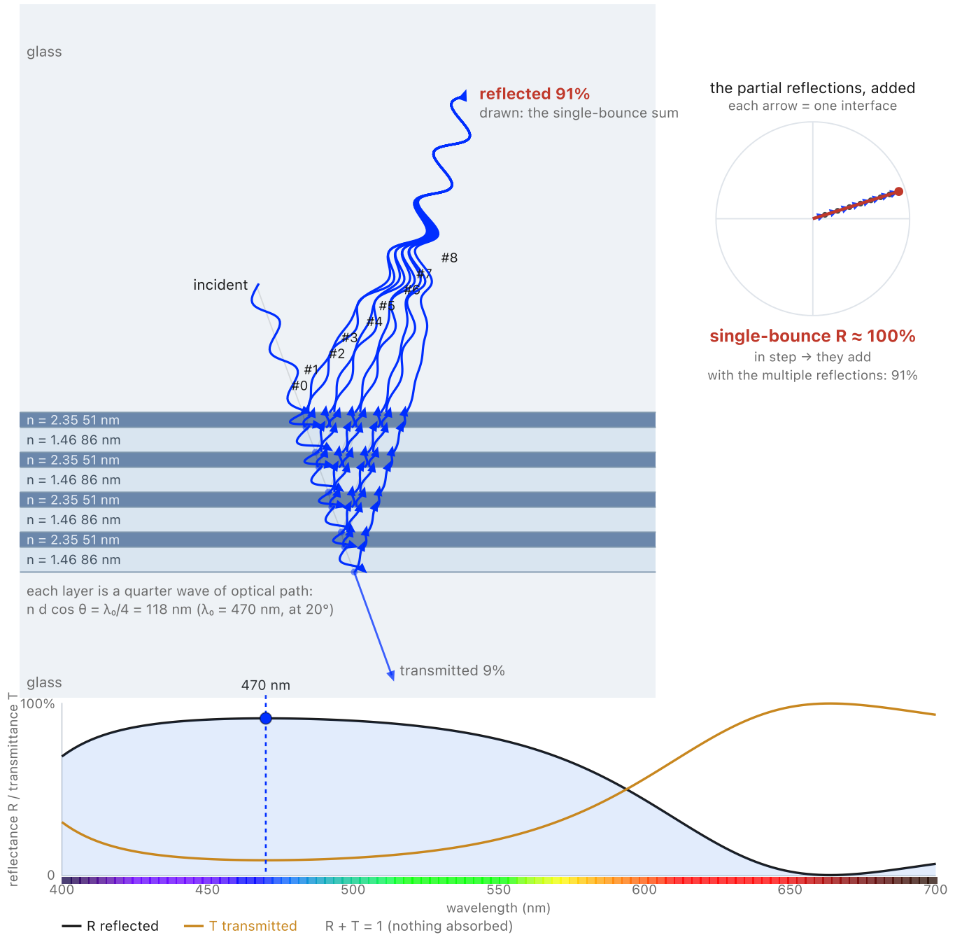
Figure 4.6.9 (reproduced). What the dichroic coating does, at the interface. The beam-splitter figures above trace whole beams through the block; here we zoom in on the coating that does the work, and cut it down to an eight-layer stack so the mechanism is visible, each layer a quarter wave at 470 nm for the stack's 20^\circ diagonal ( nd \cos \theta = \lambda_0/4 ). A single wavelength, the one control, meets the stack and you can follow it interface by interface: at each one a little reflects and the rest is transmitted, so N layers send back N + 1 partial waves, each deeper one having made an extra round trip and so returning shifted in phase. The phasor sum beside the diagram adds them tip to tail: change the wavelength, and when the round trip works out to a half wave the arrows line up and the reflections reinforce, while away from it they curl round and cancel. Even eight layers reflect 91% at 470 nm, computed exactly with the transfer-matrix method and printed beside the beams with the transmitted share; real dichroics stack
