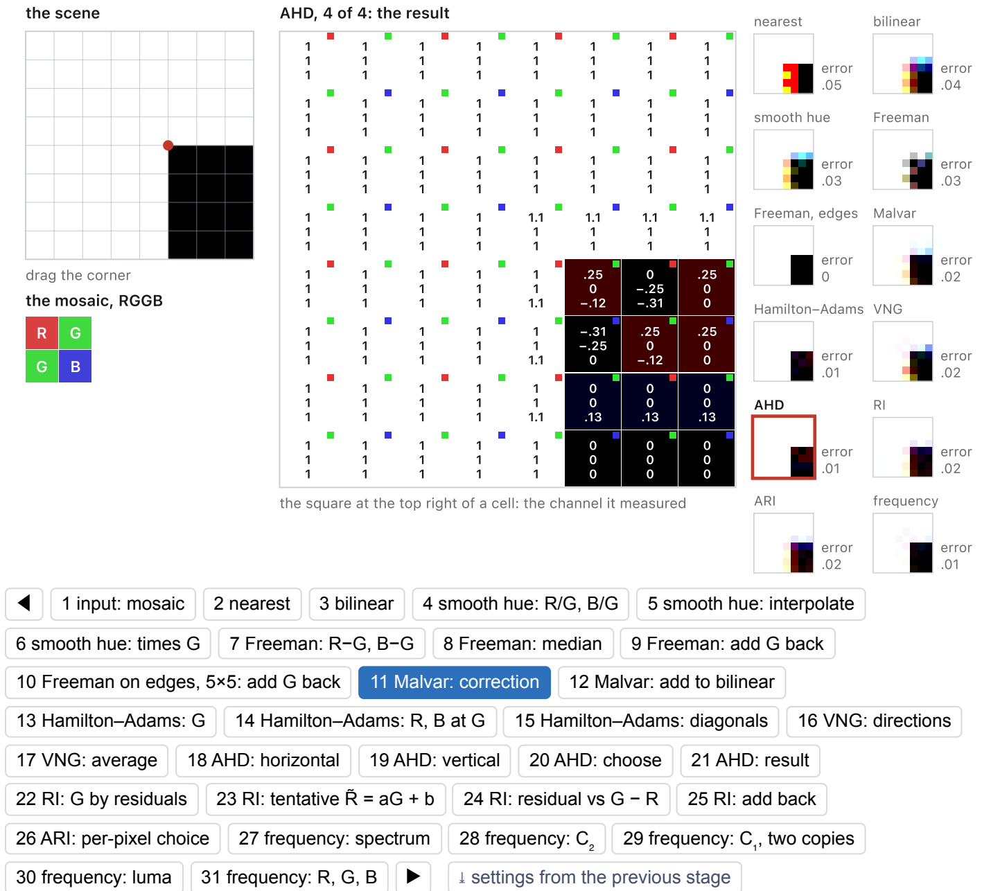
Figure 15.2.2, stage 11 (reproduced). Malvar-He-Cutler : the correction each missing channel receives, the Laplacian of the measured channel scaled by the published gains; then the bilinear estimate plus that correction. Near an edge the correction overshoots, and the values leave the range 0 to 1. Interactive: the same controls, and a checkbox that follows the result with Freeman's 5 \times 5 median; the stages step through the two steps.
